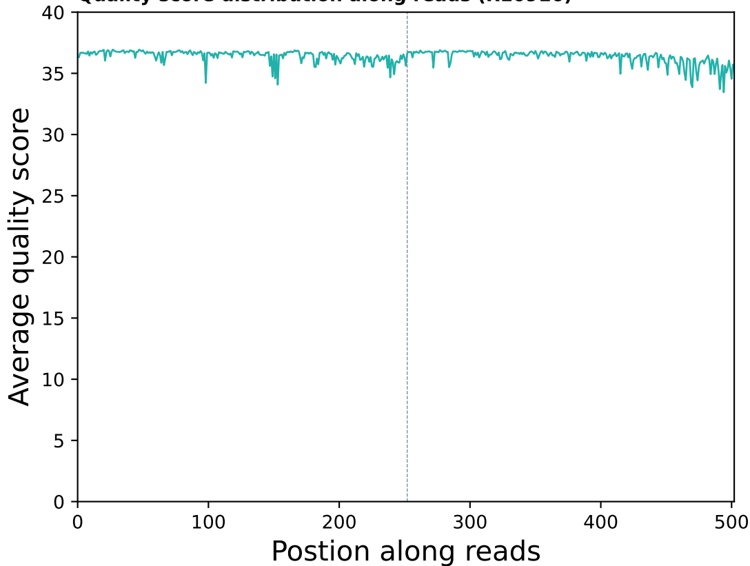
Quality score distribution along reads (R10916)
